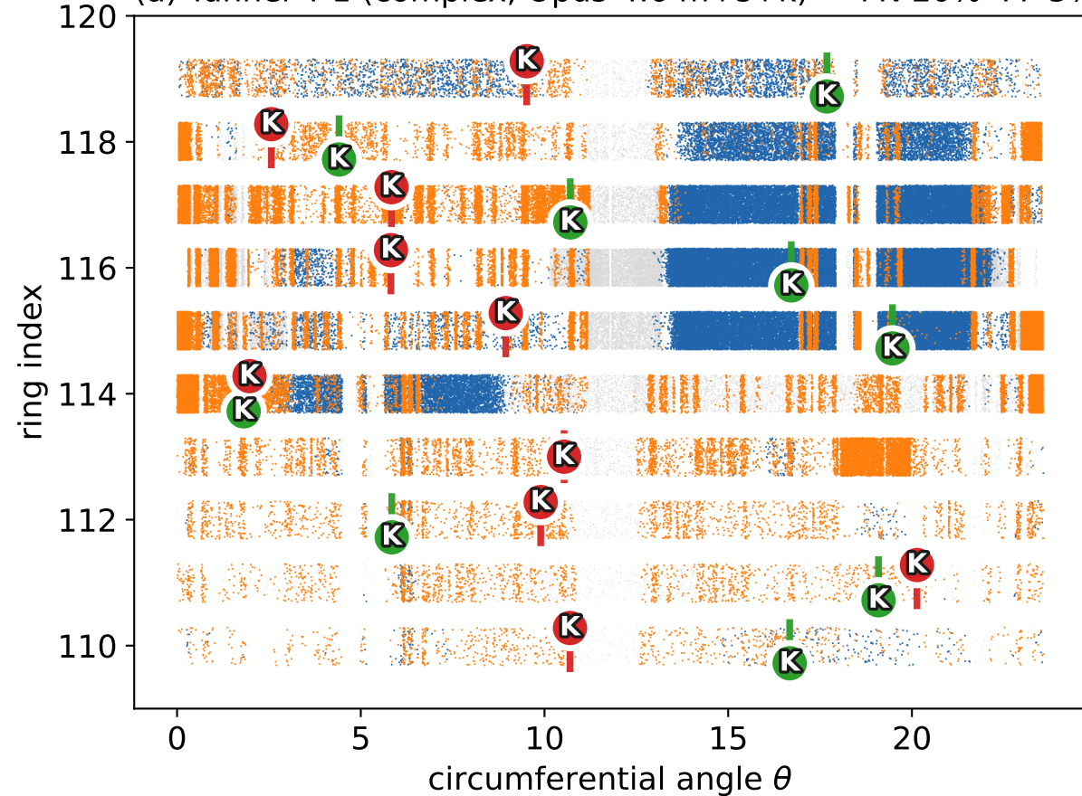
(a) Tunnel 4-1 (complex, Opus-4.6 m+s+k) — FN 20% FP 5%
