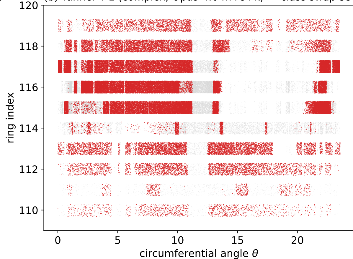
(b) Tunnel 4-1 (complex, Opus-4.6 m+s+k) — class swap 35%
